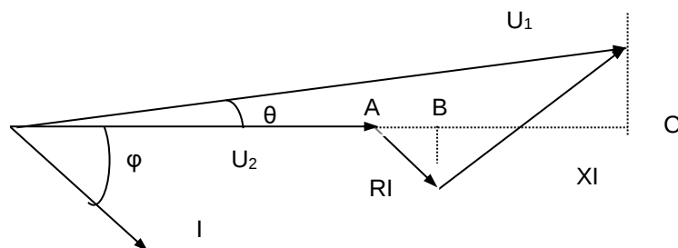
Figura 2. Diagrama vectorial.
